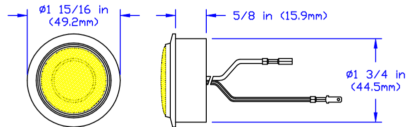
FLUSH MOUNT
