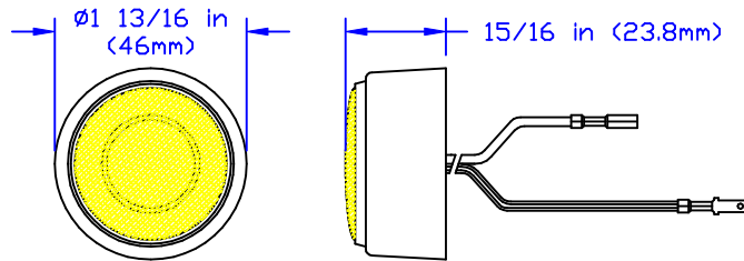
SURFACE MOUNT
